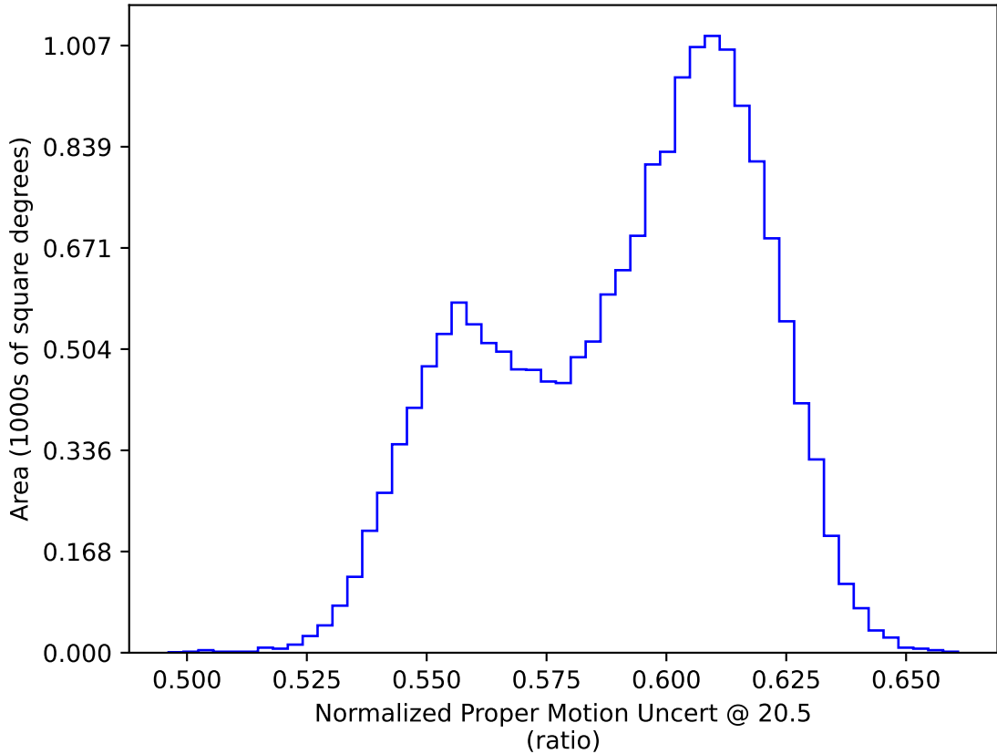
ddf_loaded_fl1_v3.4_10yrs WFD: Normalized Proper Motion Uncert @ 20.5
