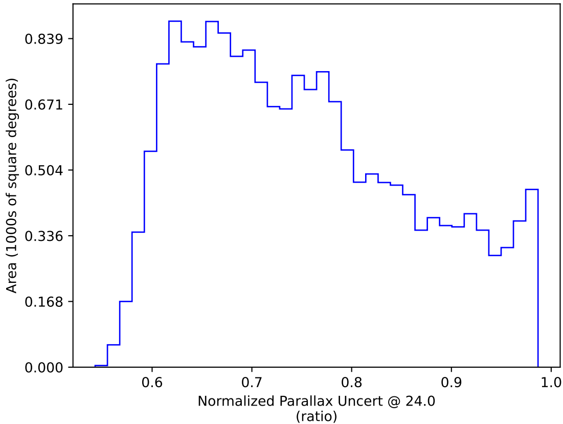
ddf_loaded_fl1_v3.4_10yrs WFD: Normalized Parallax Uncert @ 24.0
