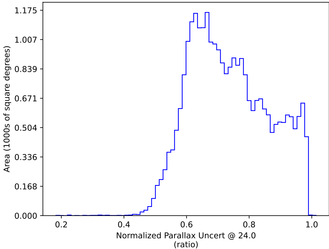
ddf_loaded_fl1_v3.4_10yrs All sky: Normalized Parallax Uncert @ 24.0
