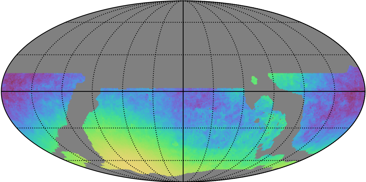
ddf_loaded_fl1_v3.4_10yrs WFD y band only: Normalized Parallax Uncert @ 21.3
