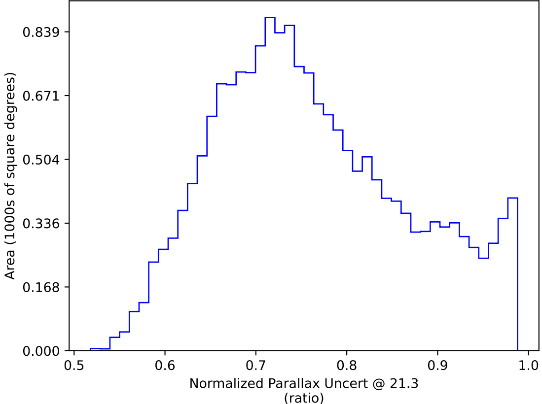
ddf_loaded_fl1_v3.4_10yrs WFD y band only: Normalized Parallax Uncert @ 21.3
