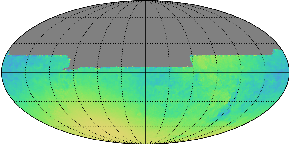
ddf_loaded_fl1_v3.4_10yrs All sky y band only: Normalized Parallax Uncert @ 21.3
