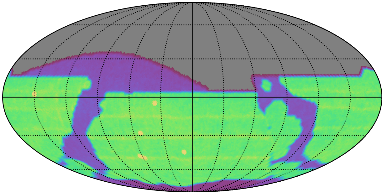
ddf_loaded_fl1_v3.4_10yrs All sky all bands: N Unique Nights
