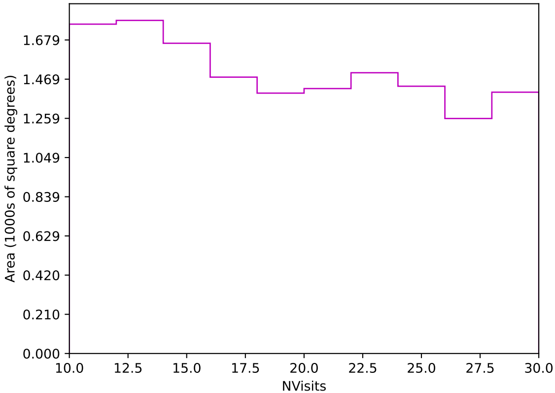
ddf_loaded_fl1_v3.4_10yrs Yr 3-4 z band: NVisits
