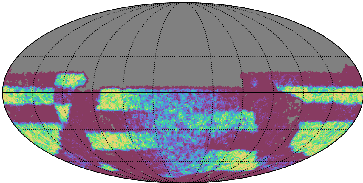
ddf_loaded_fl1_v3.4_10yrs Yr 3-4 y band: NVisits
