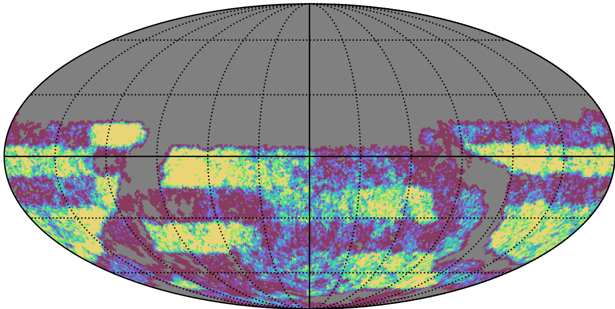
ddf_loaded_fl1_v3.4_10yrs Yr 3-4 u band: NVisits
