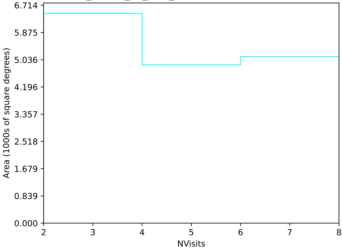
ddf_loaded_fl1_v3.4_10yrs Yr 3-4 u band: NVisits
