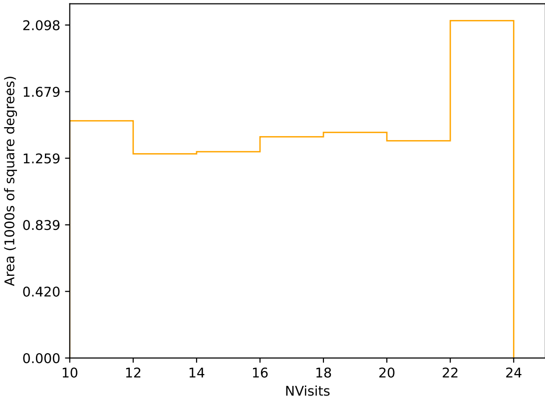
ddf_loaded_fl1_v3.4_10yrs Yr 3-4 r band: NVisits
