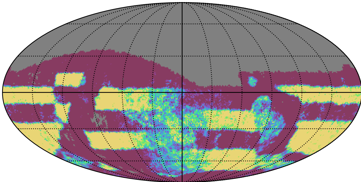
ddf_loaded_fl1_v3.4_10yrs Yr 3-4 i band: NVisits
