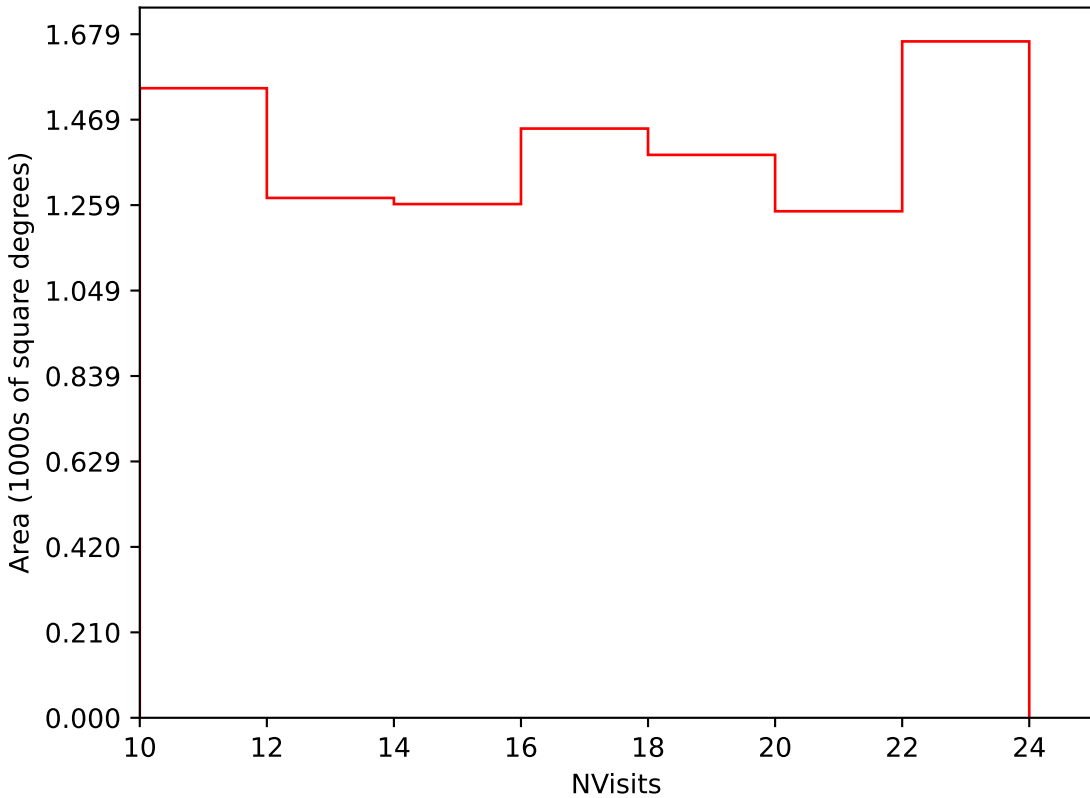
ddf_loaded_fl1_v3.4_10yrs Yr 3-4 i band: NVisits
