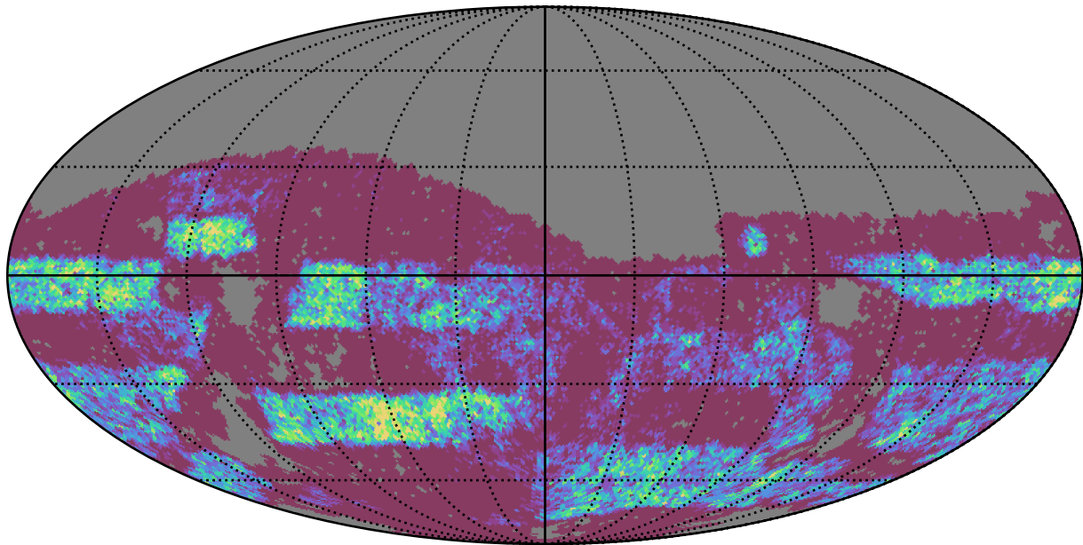
ddf_loaded_fl1_v3.4_10yrs Yr 3-4 g band: NVisits
