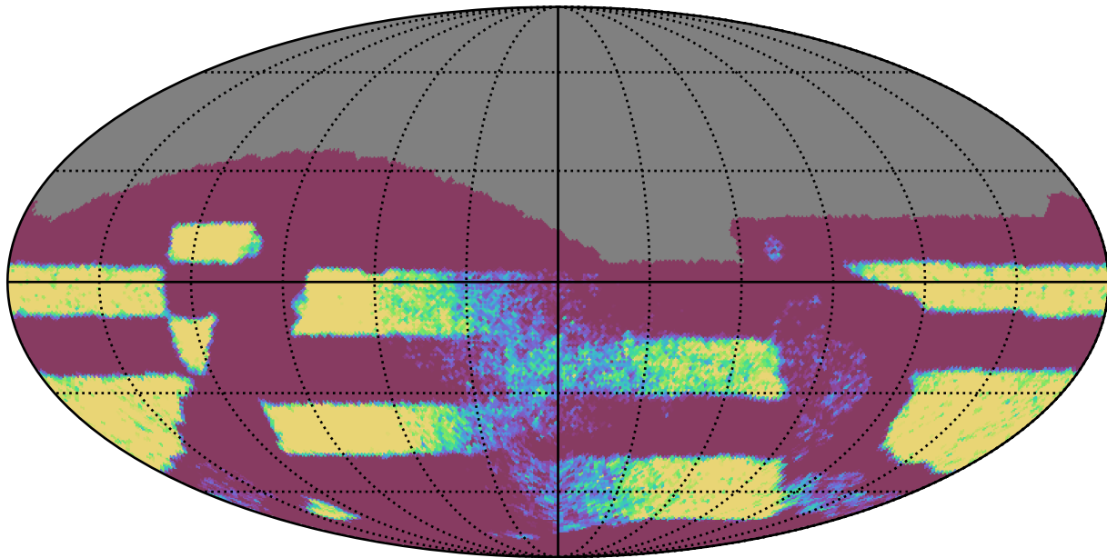
ddf_loaded_fl1_v3.4_10yrs Yr 3-4 all bands: NVisits
