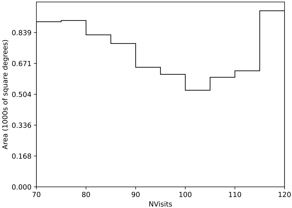
ddf_loaded_fl1_v3.4_10yrs Yr 3-4 all bands: NVisits
