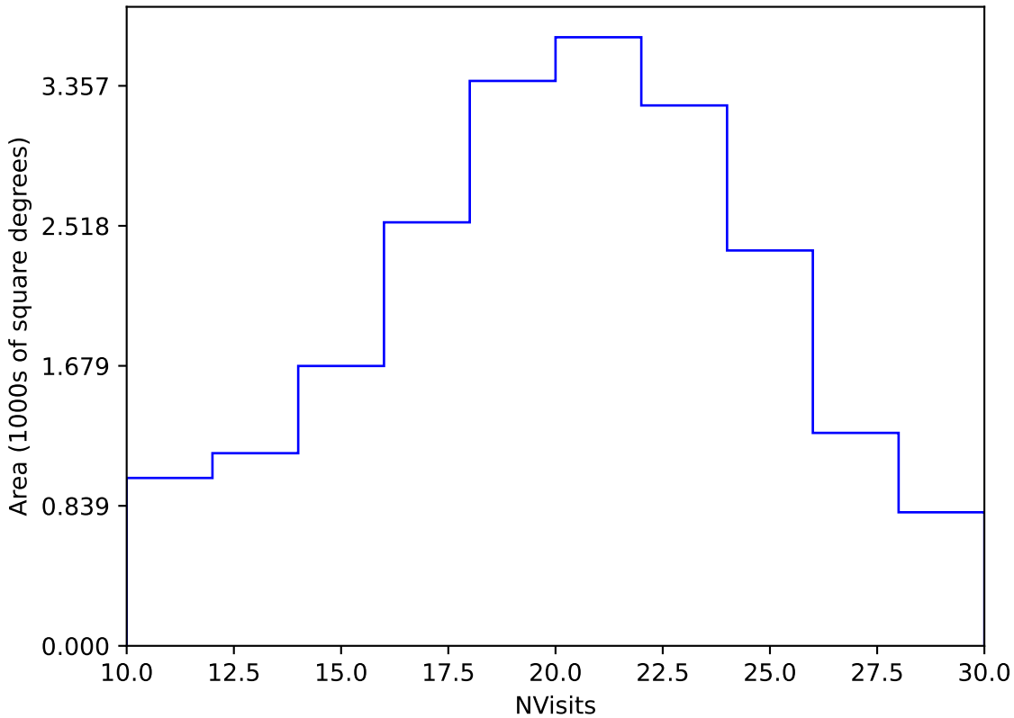
ddf_loaded_fl1_v3.4_10yrs Yr 1 y band: NVisits
