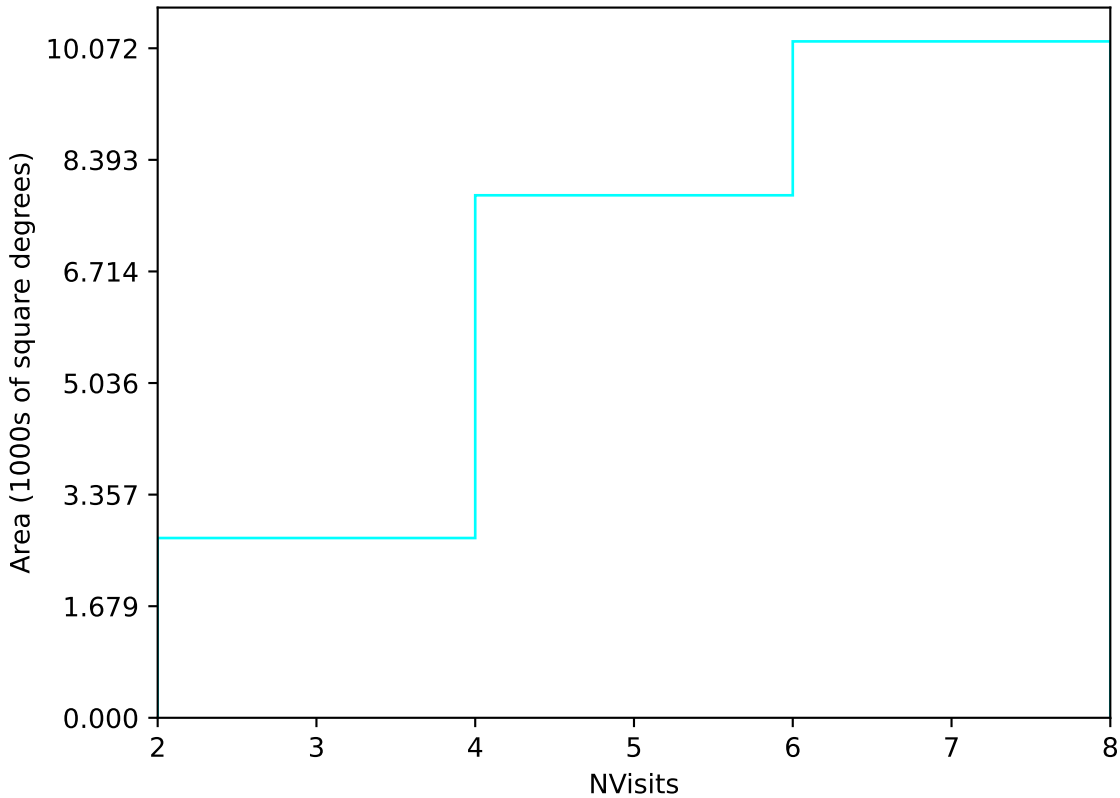
ddf_loaded_fl1_v3.4_10yrs Yr 1 u band: NVisits
