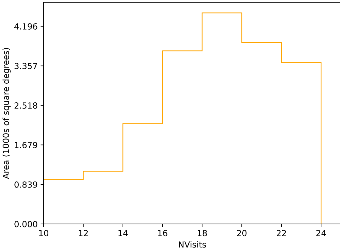
ddf_loaded_fl1_v3.4_10yrs Yr 1 r band: NVisits
