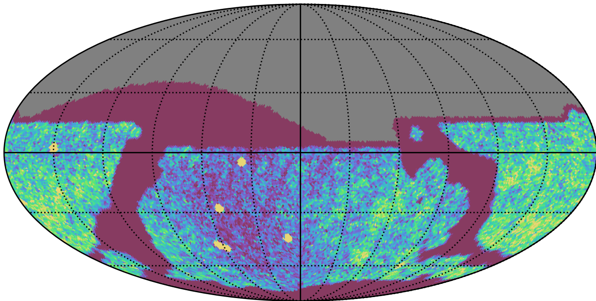
ddf_loaded_fl1_v3.4_10yrs Yr 1 all bands: NVisits
