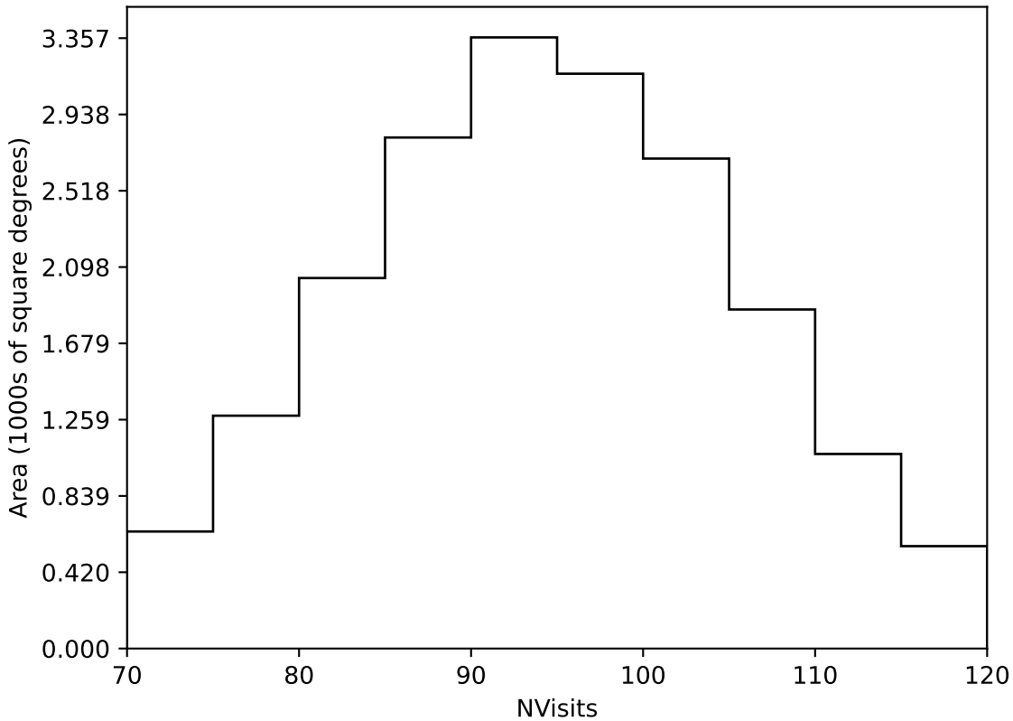
ddf_loaded_fl1_v3.4_10yrs Yr 1 all bands: NVisits
