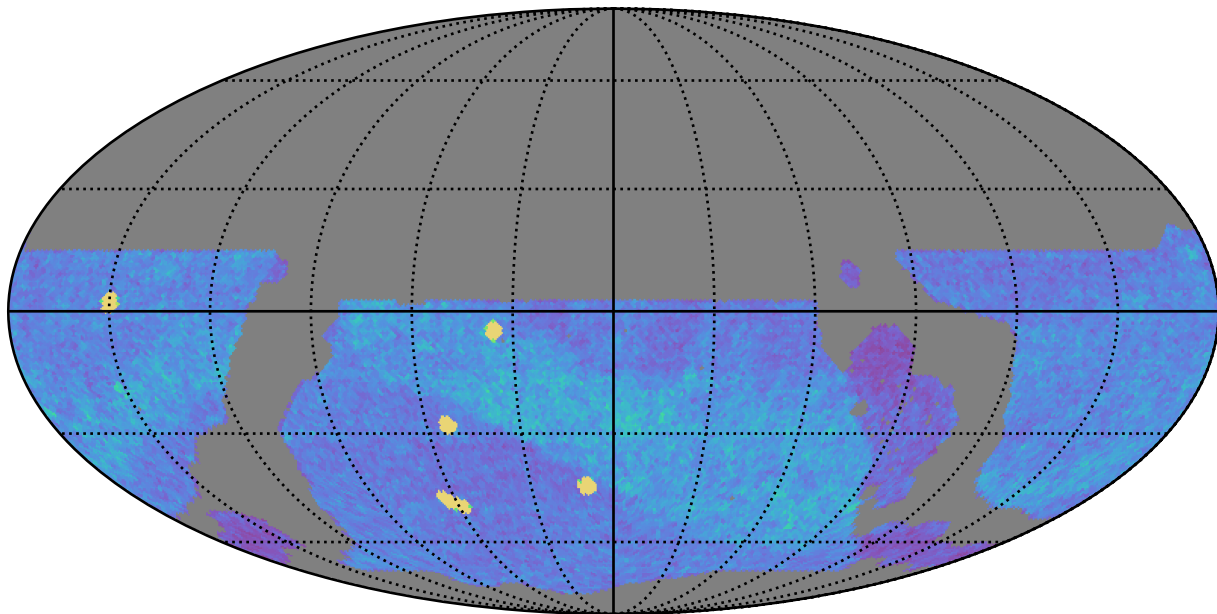
ddf_loaded_fl1_v3.4_10yrs WFD z band: NVisits
