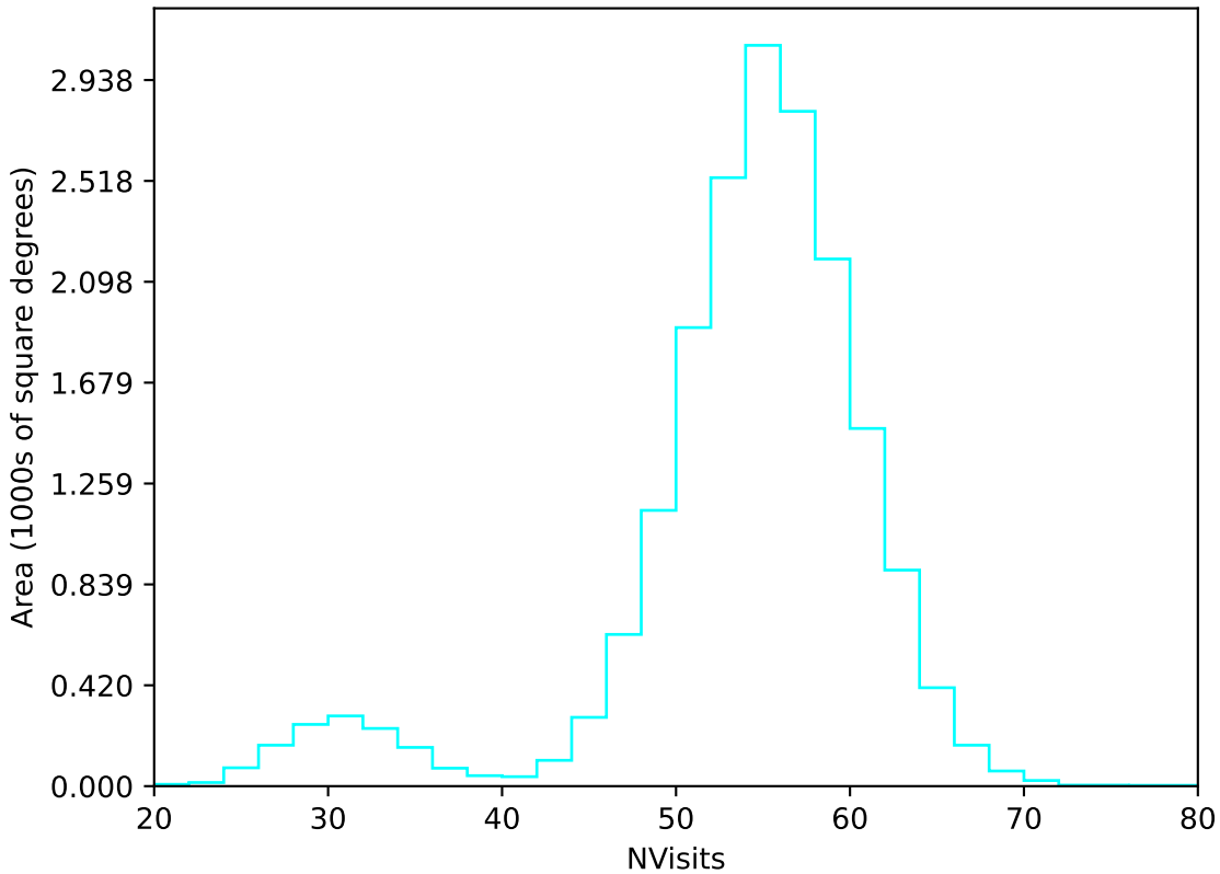
ddf_loaded_fl1_v3.4_10yrs WFD u band: NVisits
