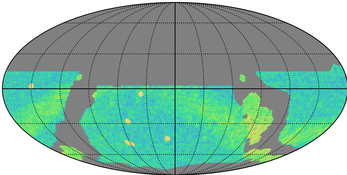
ddf_loaded_fl1_v3.4_10yrs WFD r band: NVisits
