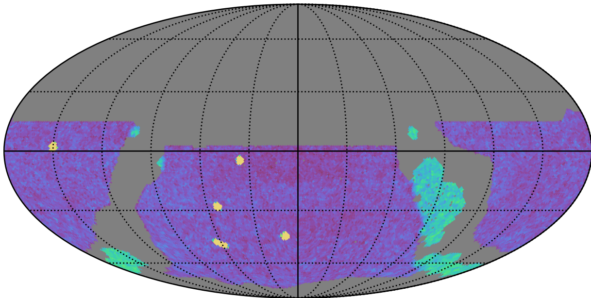
ddf_loaded_fl1_v3.4_10yrs WFD g band: NVisits
