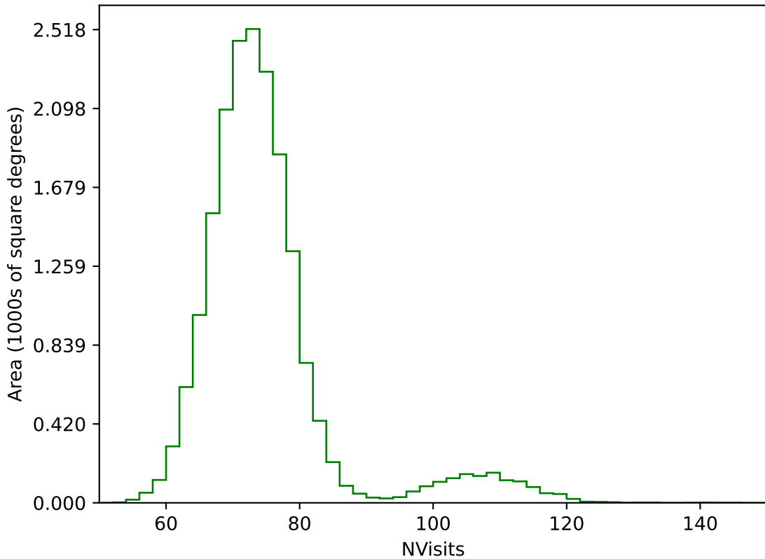
ddf_loaded_fl1_v3.4_10yrs WFD g band: NVisits
