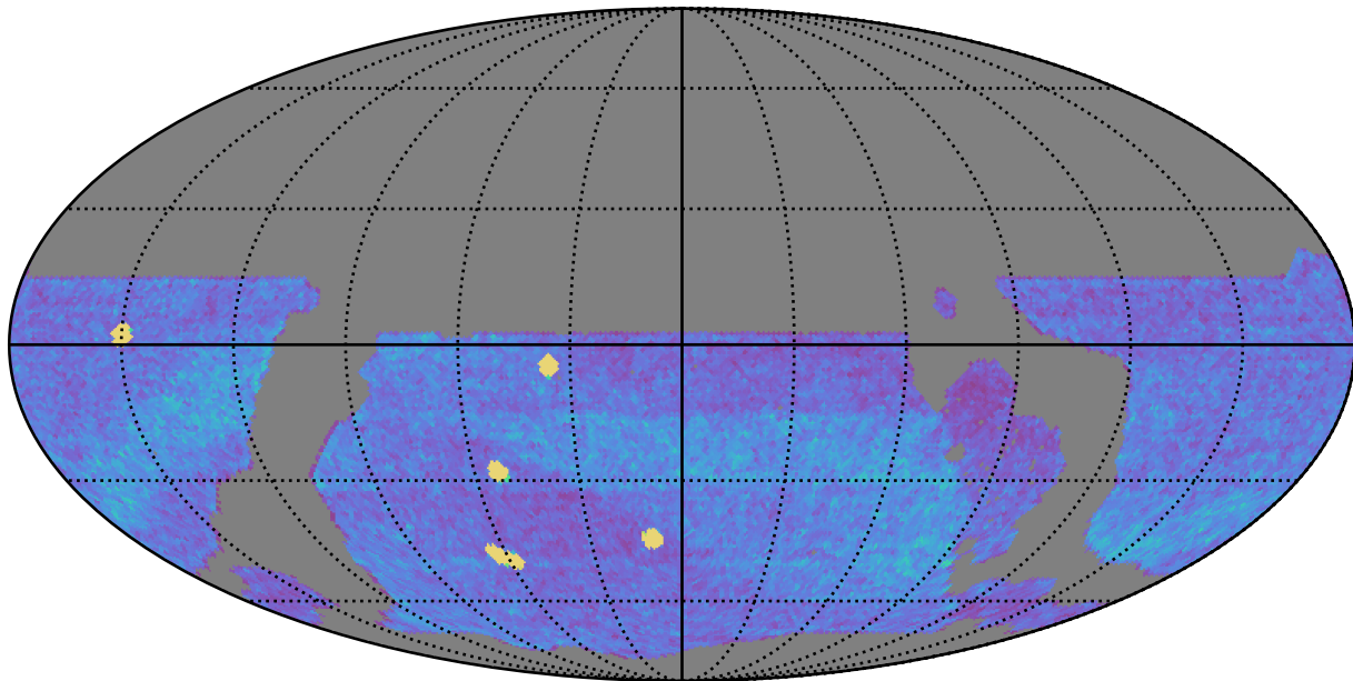
ddf_loaded_fl1_v3.4_10yrs WFD all bands: NVisits
