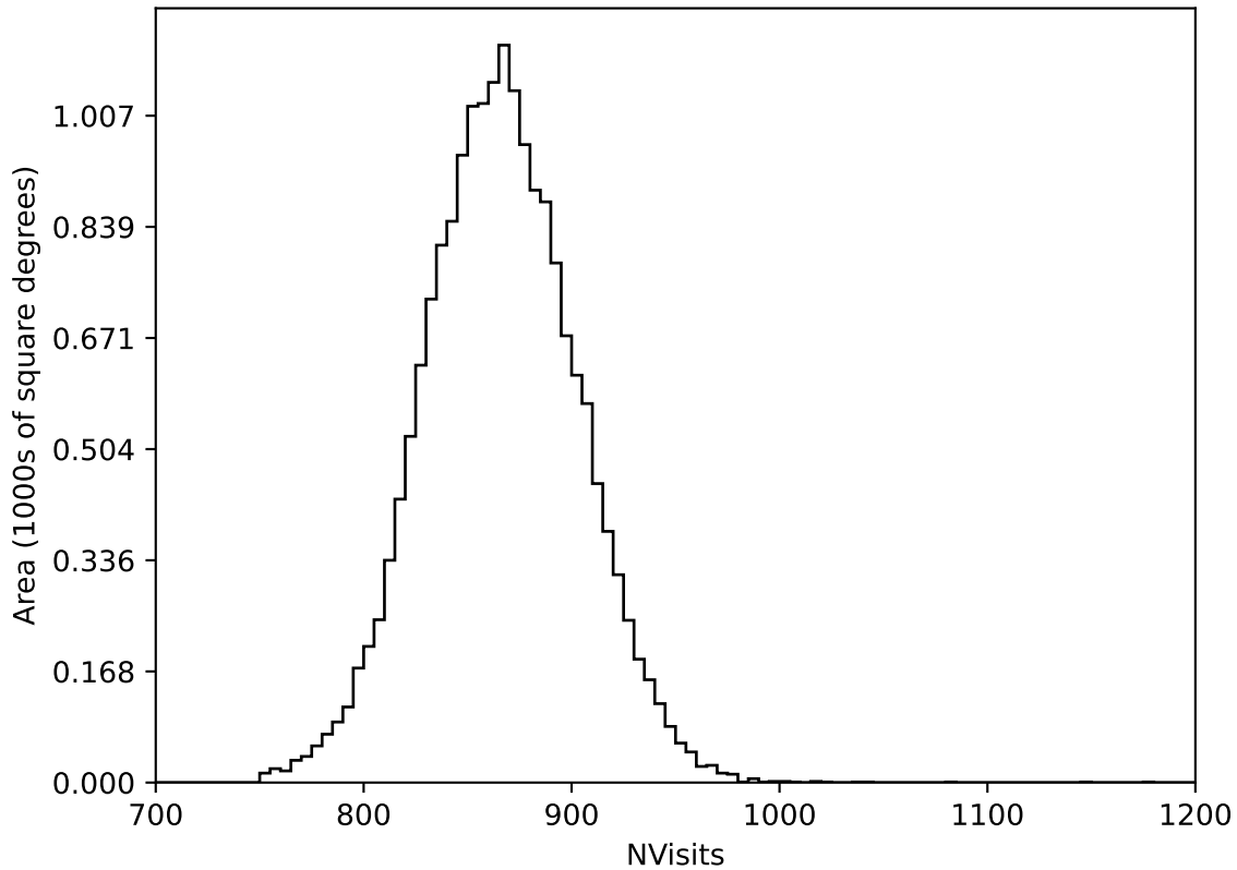
ddf_loaded_fl1_v3.4_10yrs WFD all bands: NVisits
