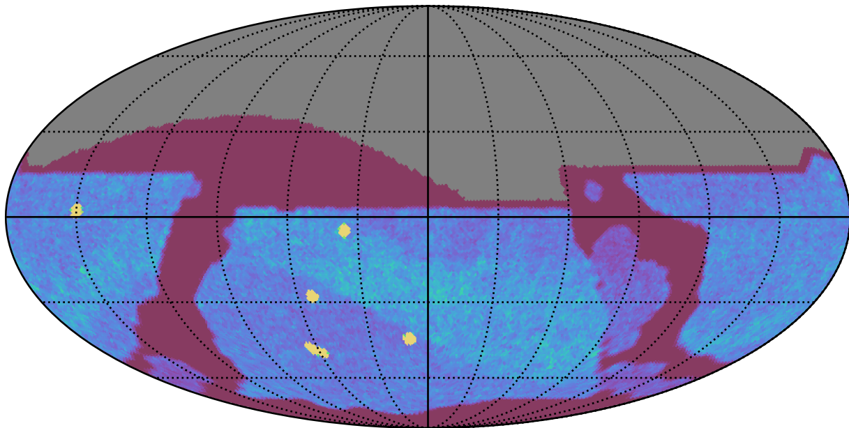
ddf_loaded_fl1_v3.4_10yrs All sky z band: NVisits
