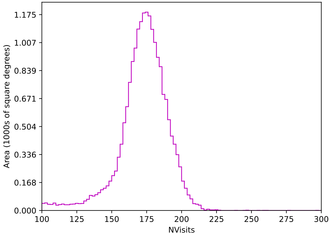
ddf_loaded_fl1_v3.4_10yrs All sky z band: NVisits
