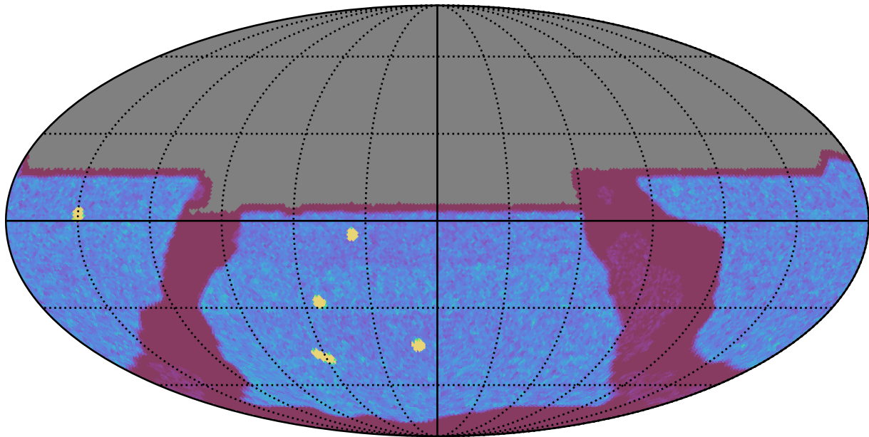
ddf_loaded_fl1_v3.4_10yrs All sky y band: NVisits
