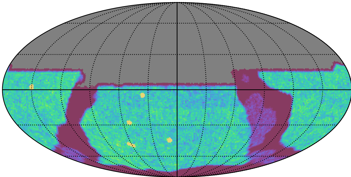
ddf_loaded_fl1_v3.4_10yrs All sky u band: NVisits
