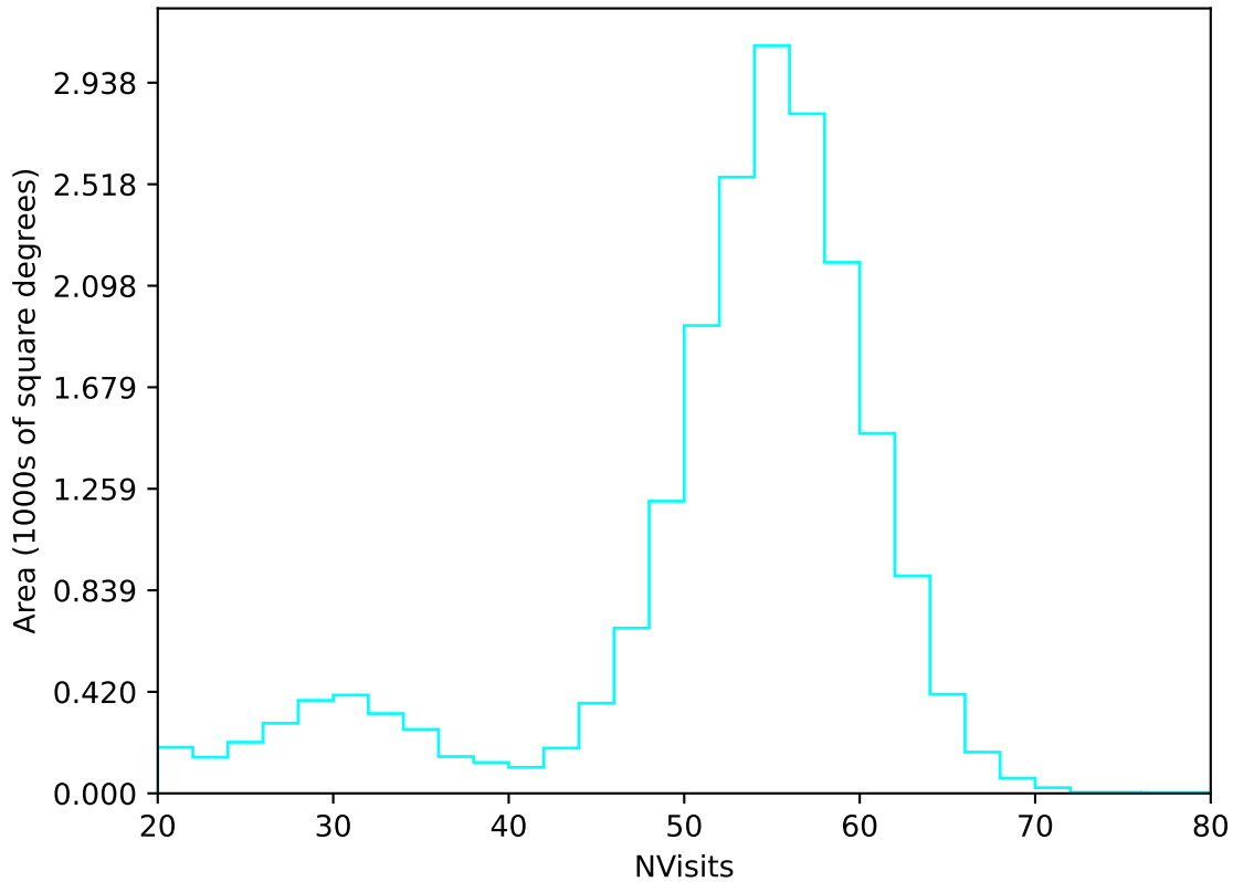
ddf_loaded_fl1_v3.4_10yrs All sky u band: NVisits
