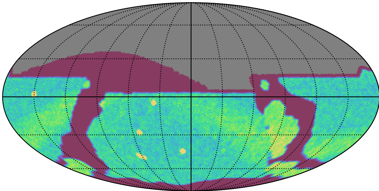
ddf_loaded_fl1_v3.4_10yrs All sky r band: NVisits
