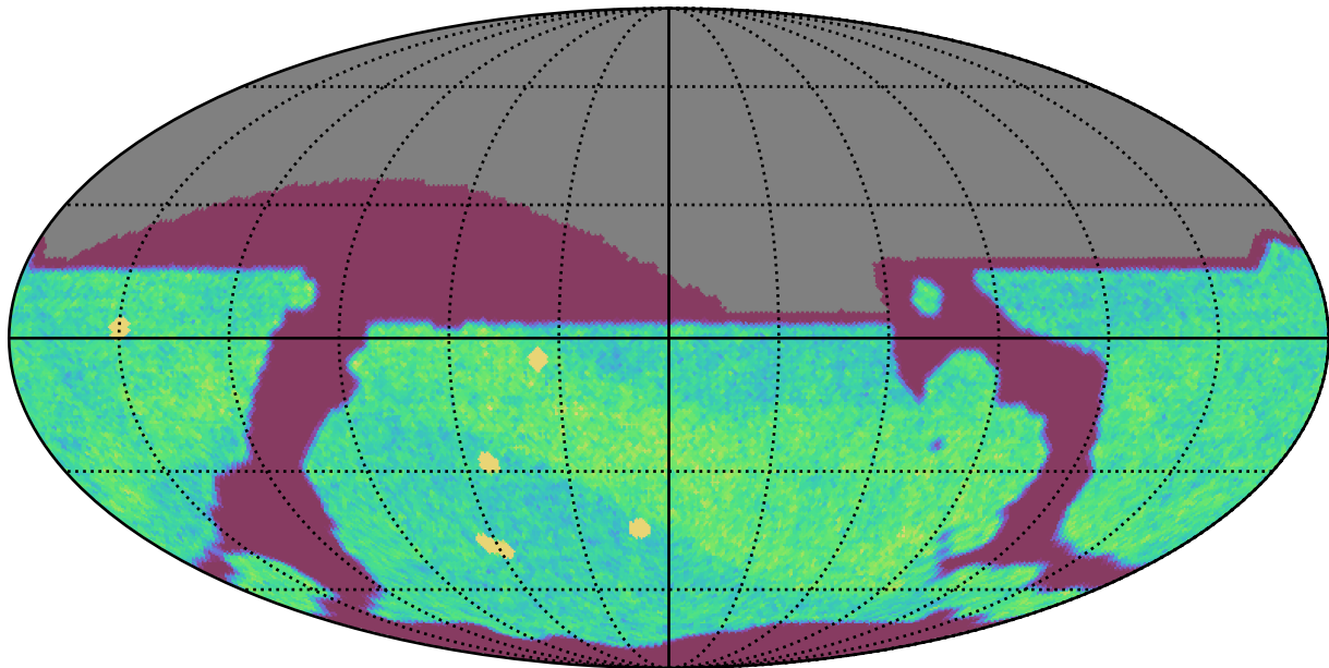
ddf_loaded_fl1_v3.4_10yrs All sky i band: NVisits
