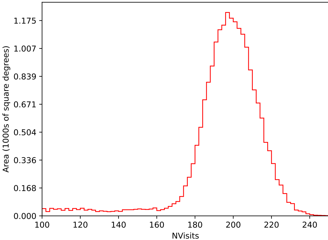
ddf_loaded_fl1_v3.4_10yrs All sky i band: NVisits
