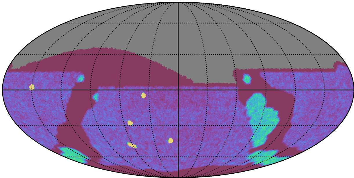
ddf_loaded_fl1_v3.4_10yrs All sky g band: NVisits
