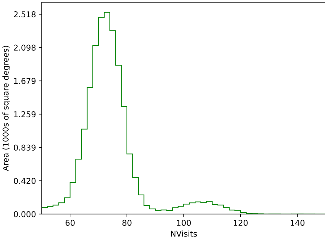
ddf_loaded_fl1_v3.4_10yrs All sky g band: NVisits
