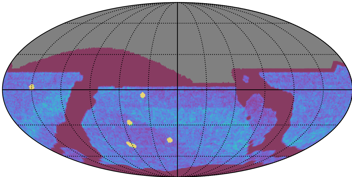
ddf_loaded_fl1_v3.4_10yrs All sky all bands: NVisits
