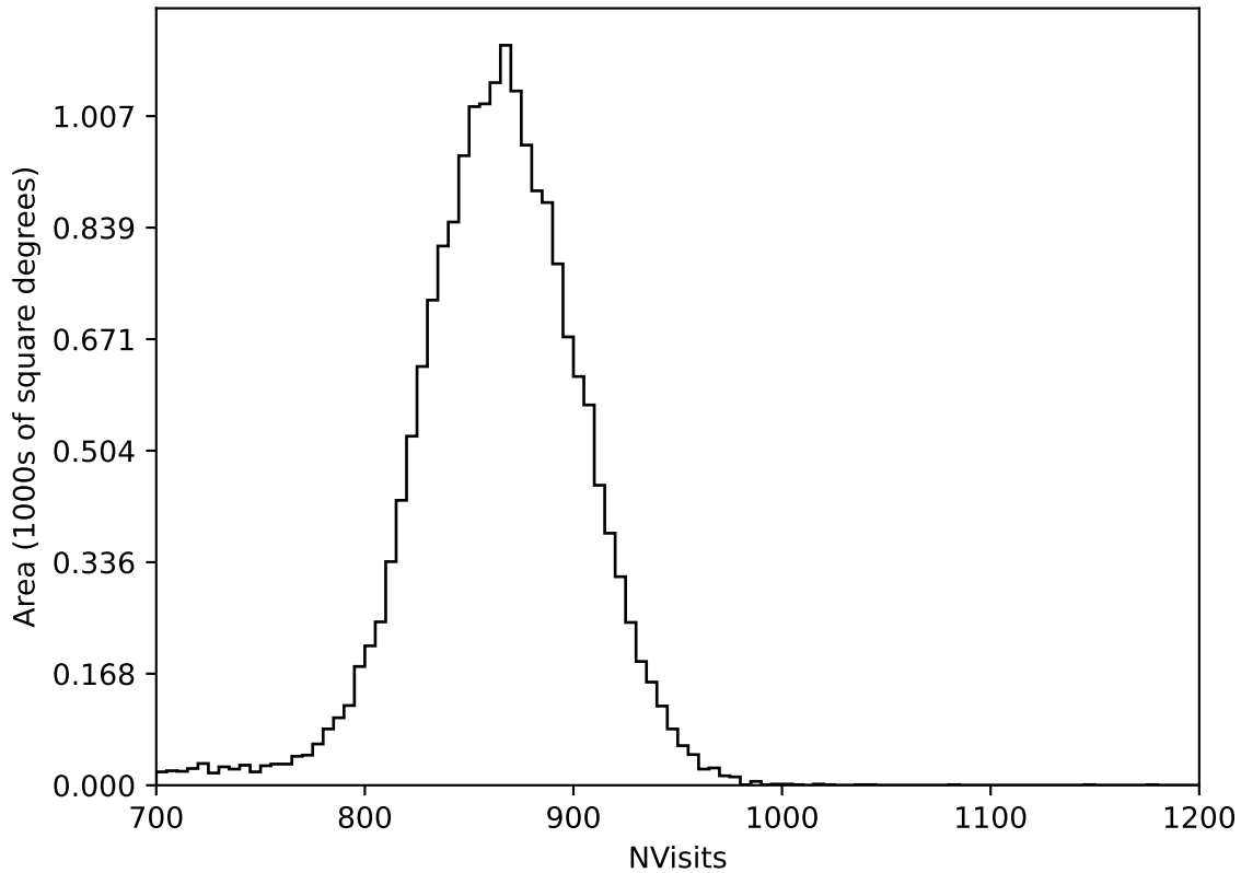
ddf_loaded_fl1_v3.4_10yrs All sky all bands: NVisits
