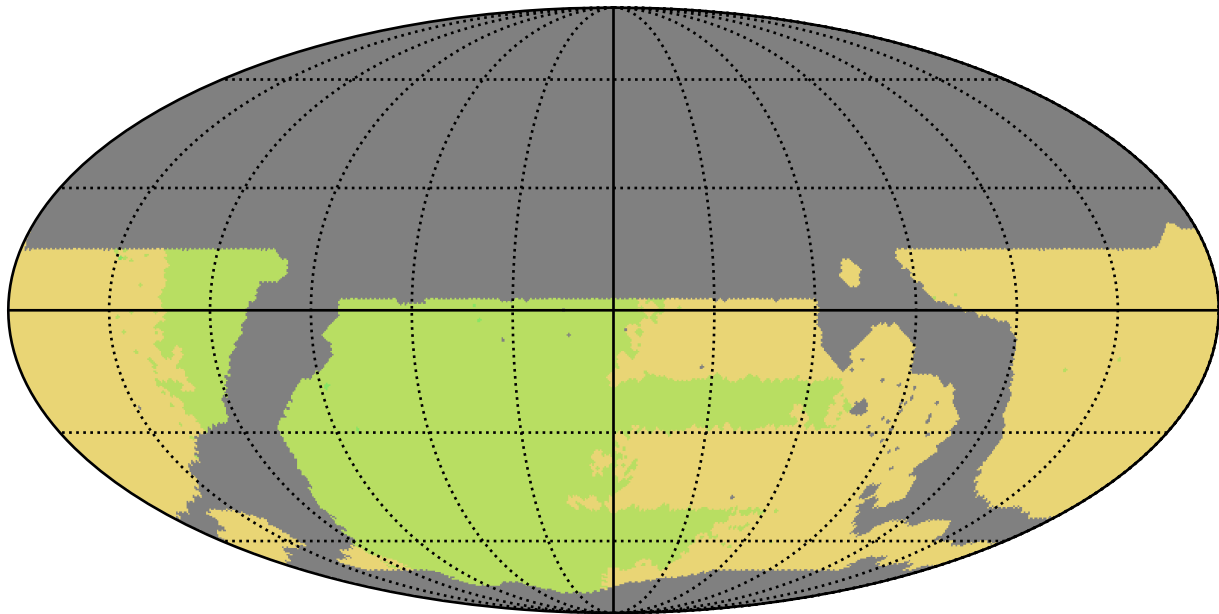
ddf_loaded_fl1_v3.4_10yrs WFD all bands: NSeasons
