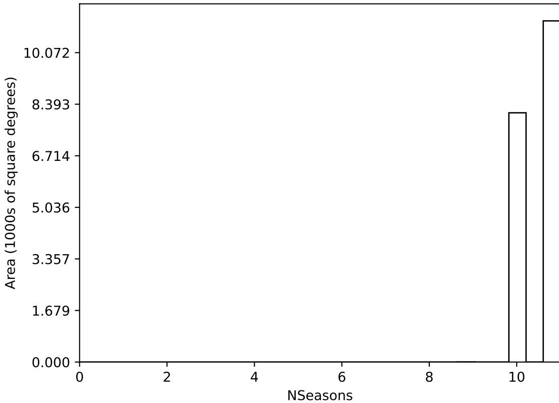
ddf_loaded_fl1_v3.4_10yrs WFD all bands: NSeasons
