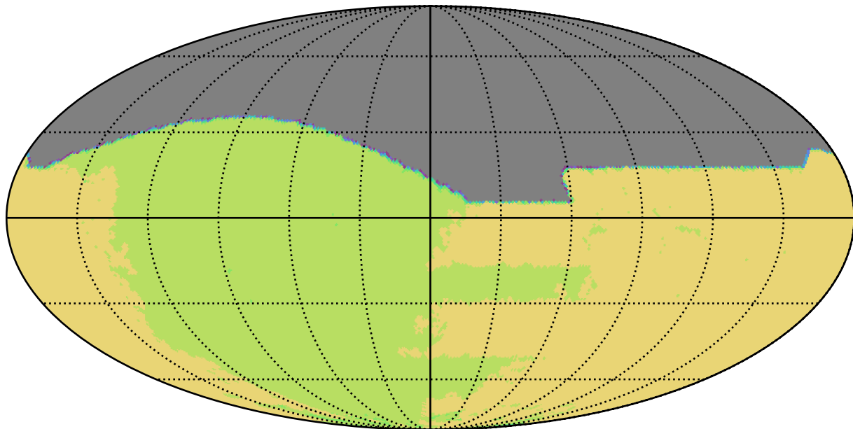
ddf_loaded_fl1_v3.4_10yrs All sky all bands: NSeasons
