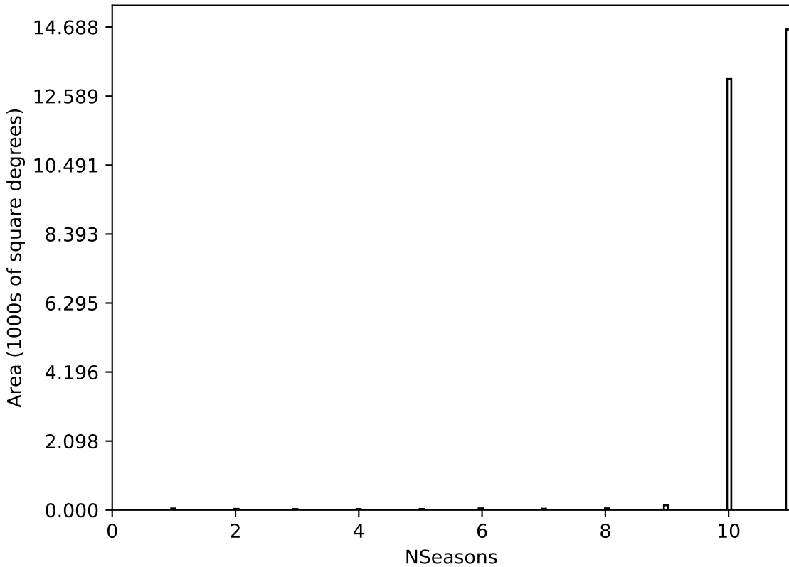
ddf_loaded_fl1_v3.4_10yrs All sky all bands: NSeasons
