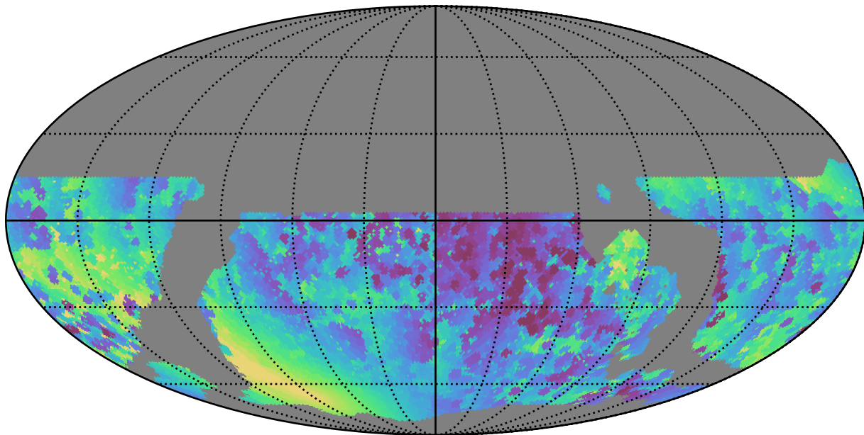
ddf_loaded_fl1_v3.4_10yrs WFD y band: Min solarElong
