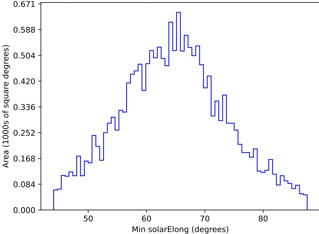
ddf_loaded_fl1_v3.4_10yrs WFD y band: Min solarElong
