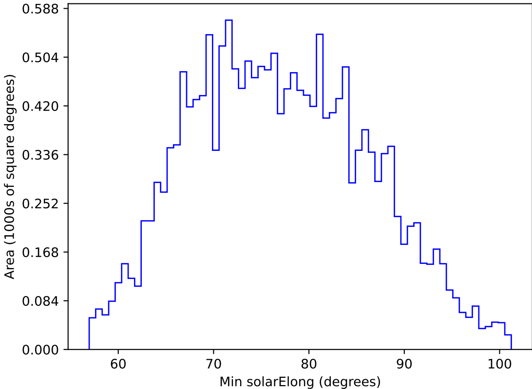
ddf_loaded_fl1_v3.4_10yrs WFD u band: Min solarElong
