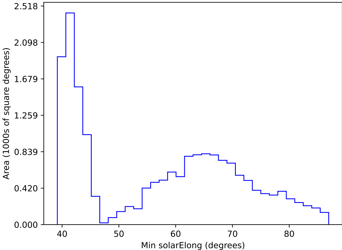
ddf_loaded_fl1_v3.4_10yrs WFD r band: Min solarElong
