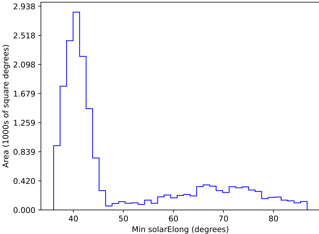
ddf_loaded_fl1_v3.4_10yrs WFD i band: Min solarElong
